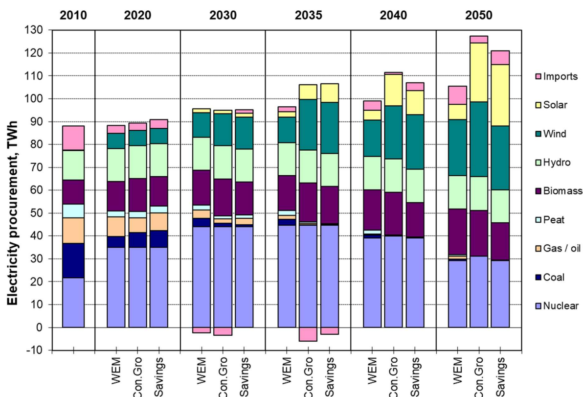
Figure 8. Electricity supply by source under different scenarios.
