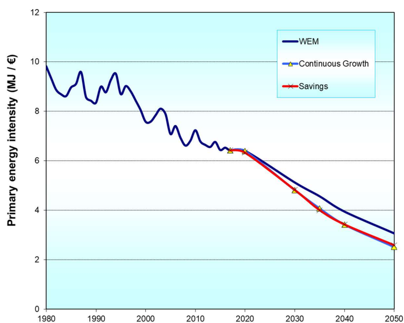
Figure 19. Trends in economic energy intensity under the WEM scenario and in the low-emission scenarios.
