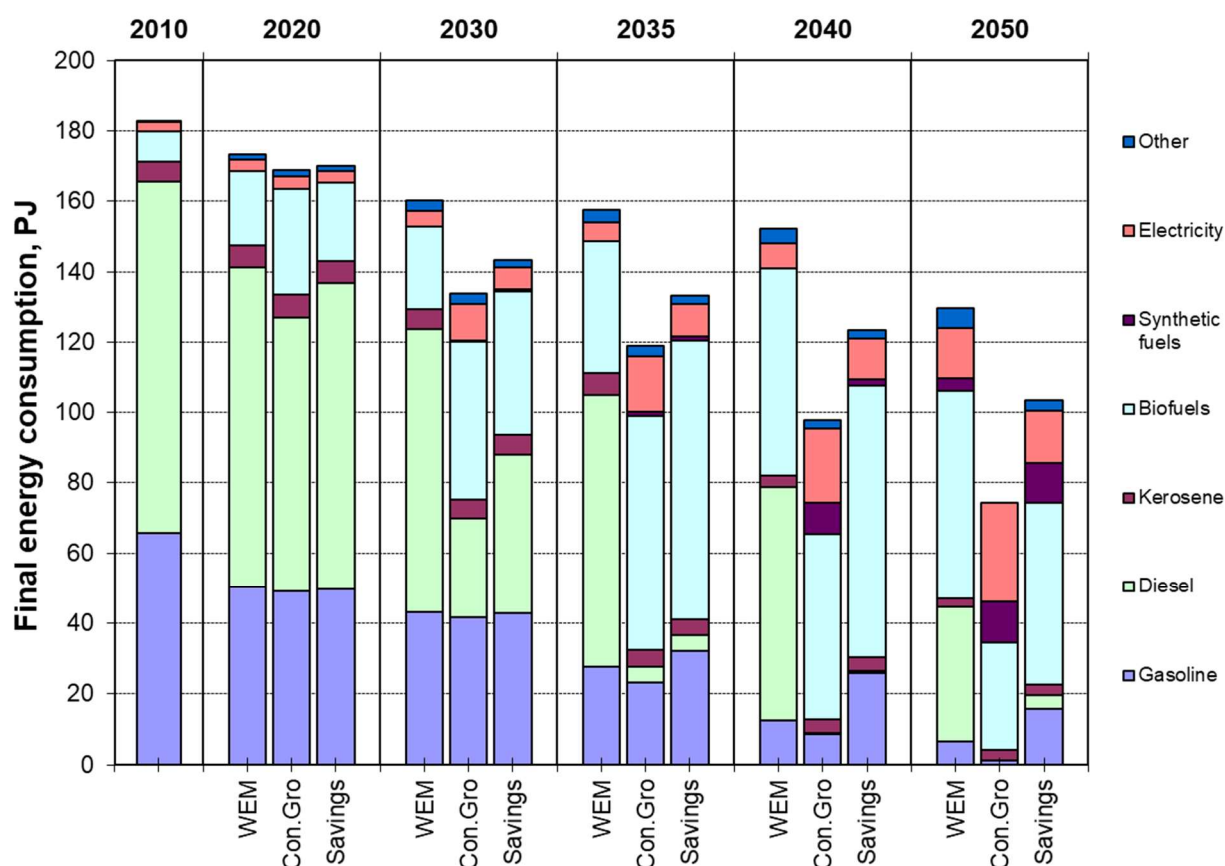
Figure 12. Modelled distribution of transport fuels by scenario.
