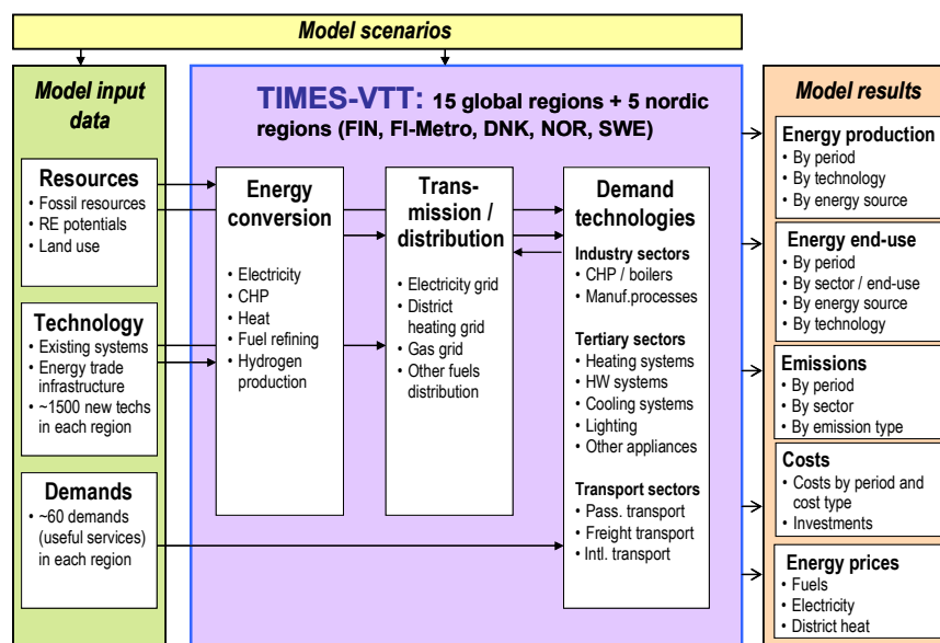
Figure 1. The TIMES model components and a simplified structure diagram for one region. The diagram describes trade in key energy commodities between regions.
