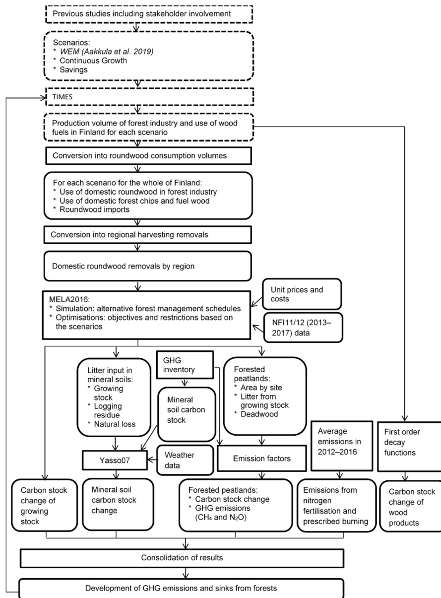
Figure 2. Calculation steps to forecast trends in forest GHG emissions and removals.
