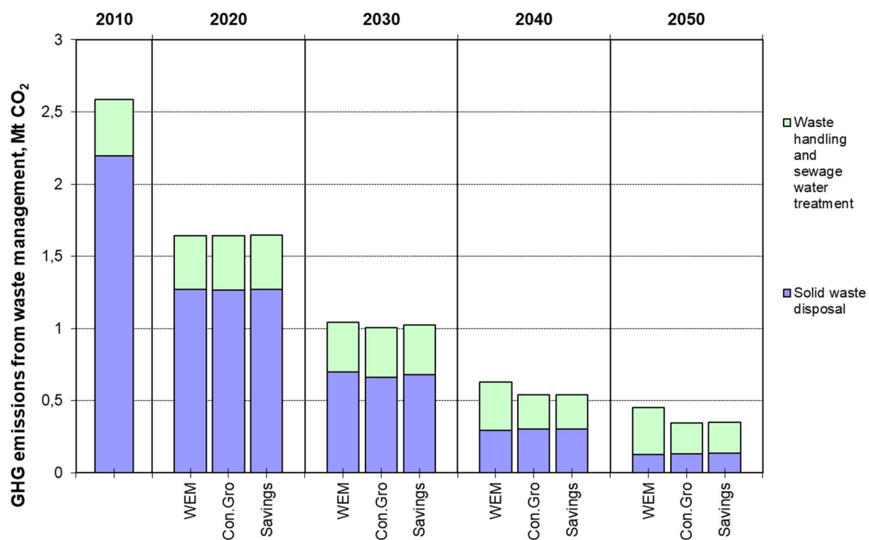
Figure 14. GHG emissions from waste management by scenario.
