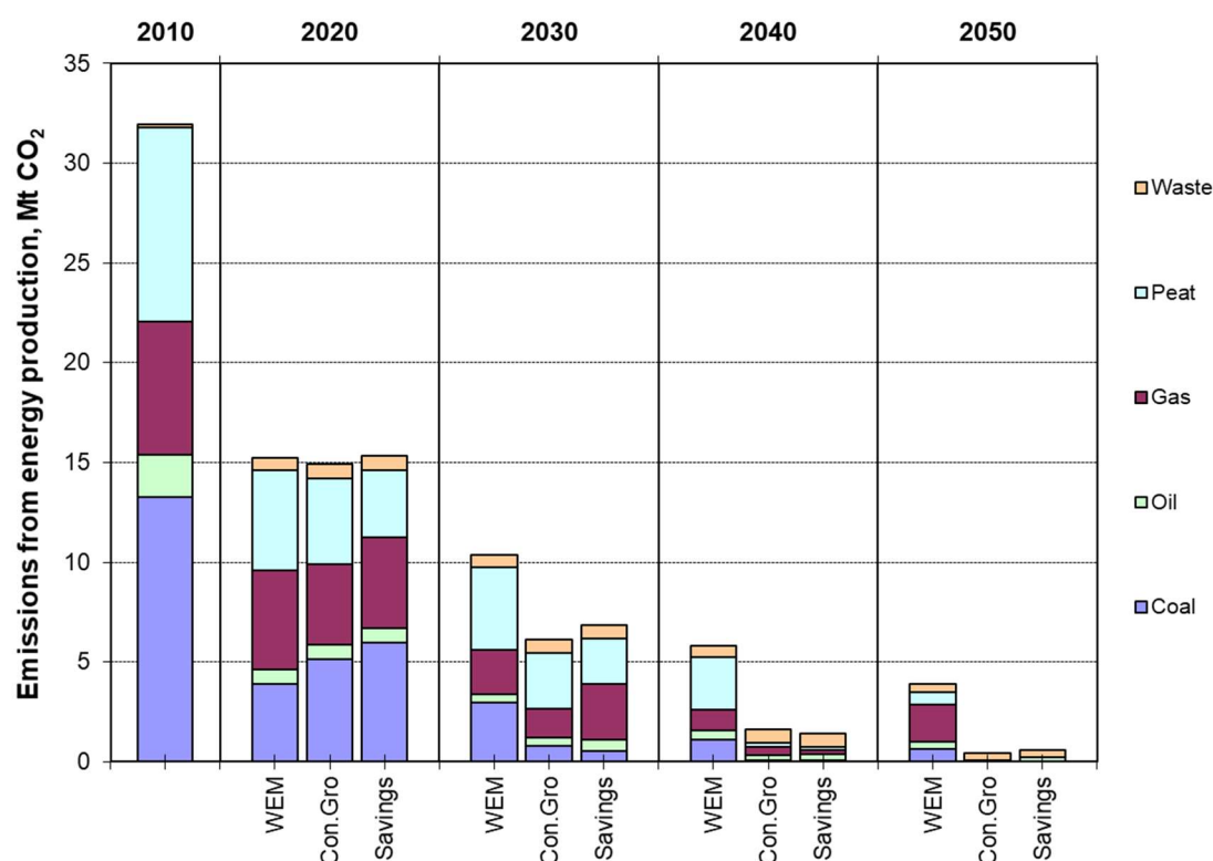
Figure 7. Development of CO 2 emissions from energy production under different scenarios.
