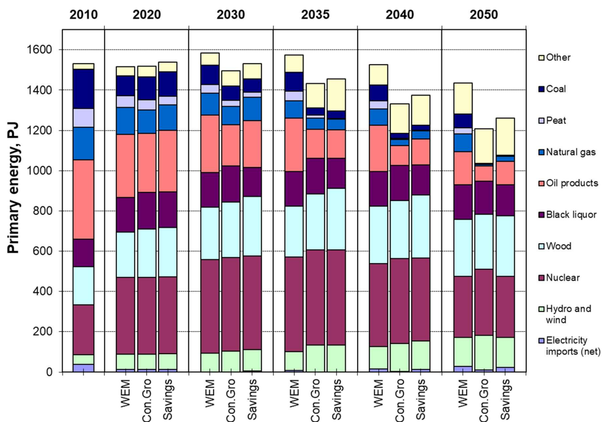
Figure 6. Modelled trends in total primary energy supply by scenario.
