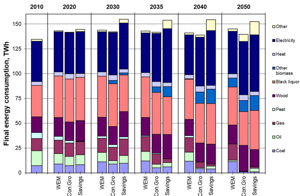
Figure 10. Final energy consumption in industry by scenario ('Other' covers hydrogen, synthetic fuels, etc.).
